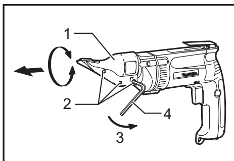
► 1. Cutting head 2. Screws 3. Loosen 4. Hex wrench
